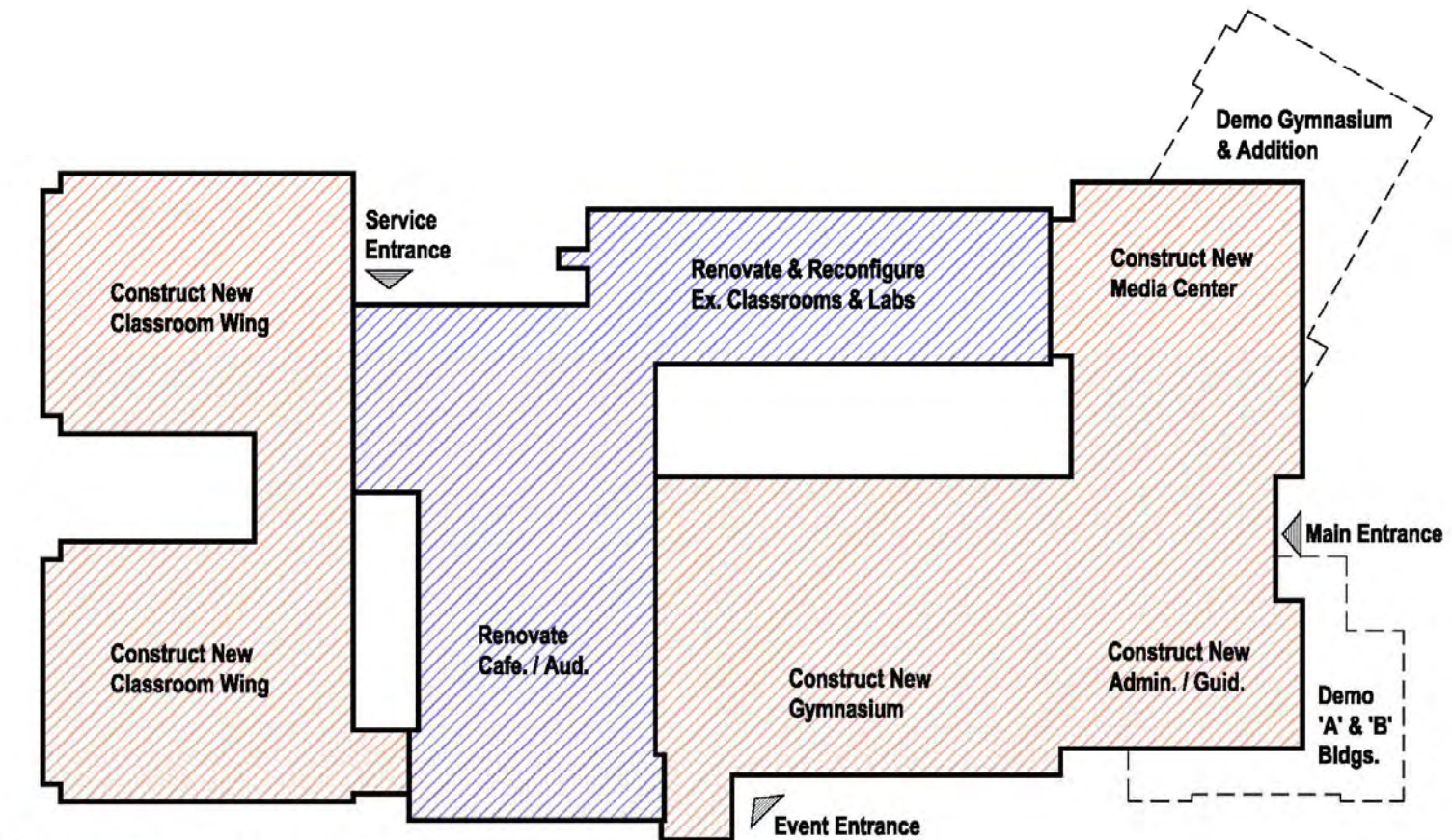
SHS Option B3 Floor Plan
